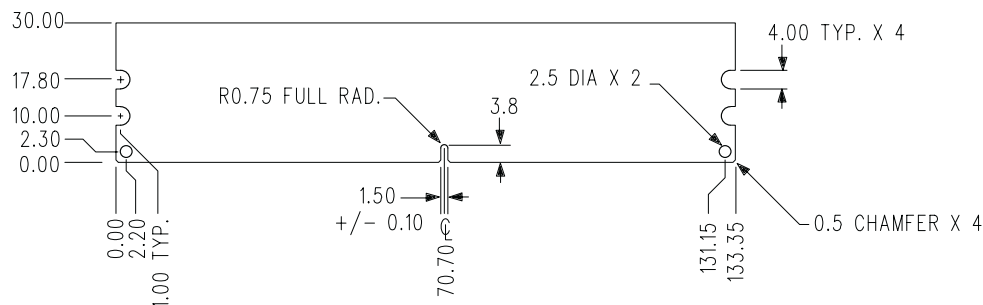
SOLDER SIDE—MIRRORED
