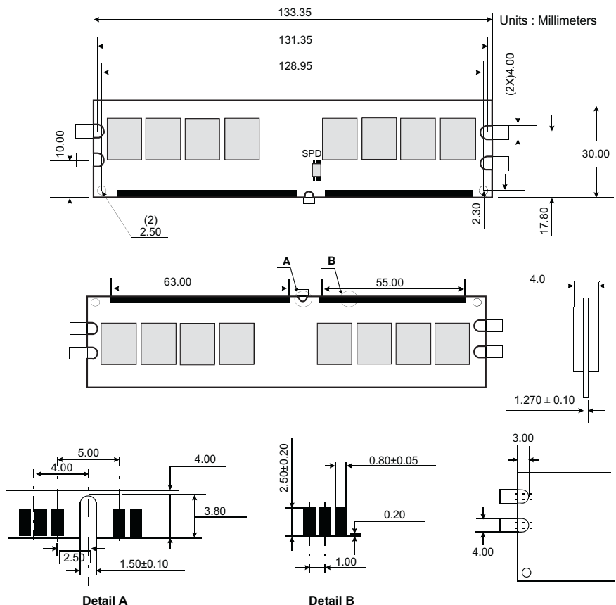
Figure 1: KVR667D2/1GR 240-Pin DIMM
