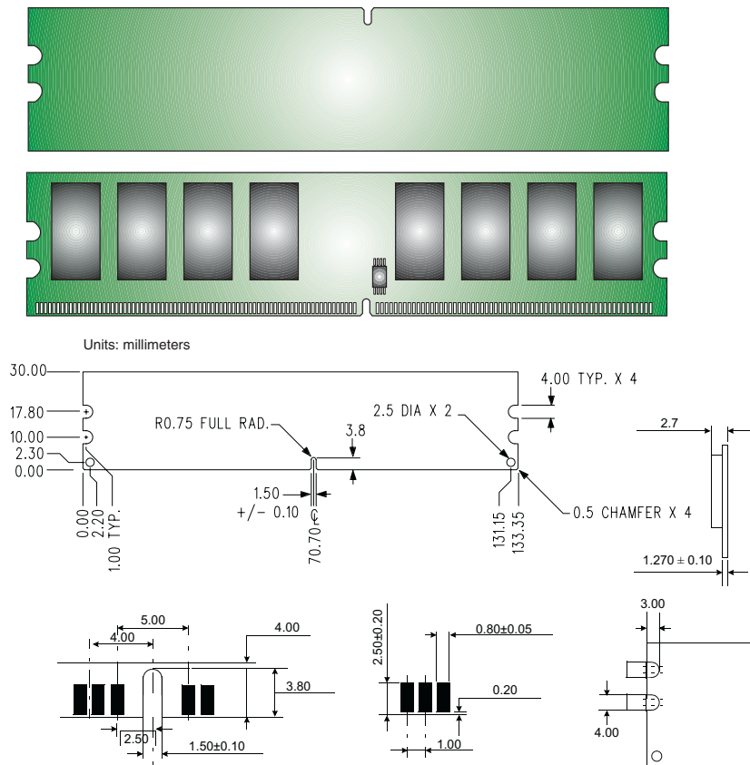
Figure 1: KVR800D2N5/512 240-Pin DIMM
