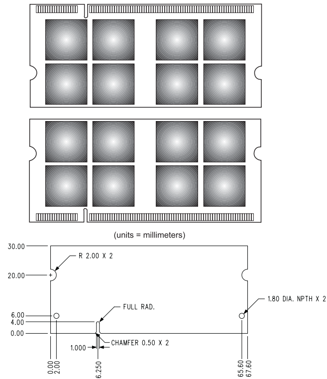
Figure 1: KVR667D2S5K2/4G 200-Pin SODIMM
