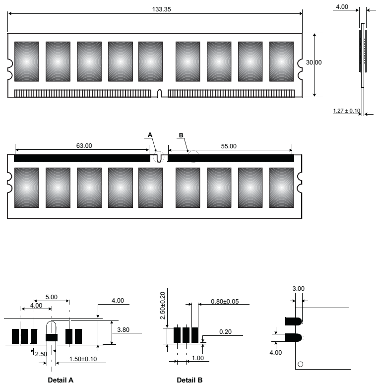
Figure 1: KVR667D2E5/4G 240-Pin DIMM
