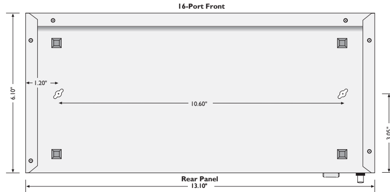
Fig. E-1 Mounting Template specifications
