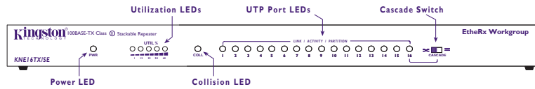
Fig. 1-2 KNE16TX/SE Front Panel
