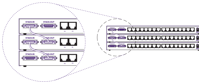
Figure 1-6 Stacking Configuration
