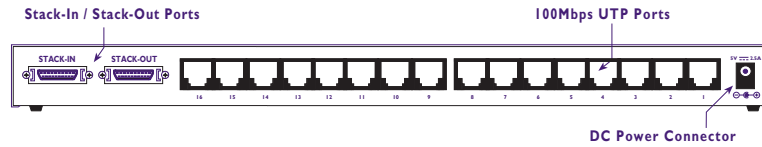
Fig. 1-4 KN16TX/SE Rear Panel
