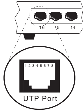
Fig. A-1 RJ-45 Connector Pin Numbers
