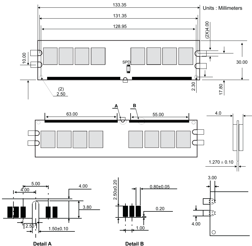
Figure 1: KVR400D2N3K2/4G 240-Pin DIMM
