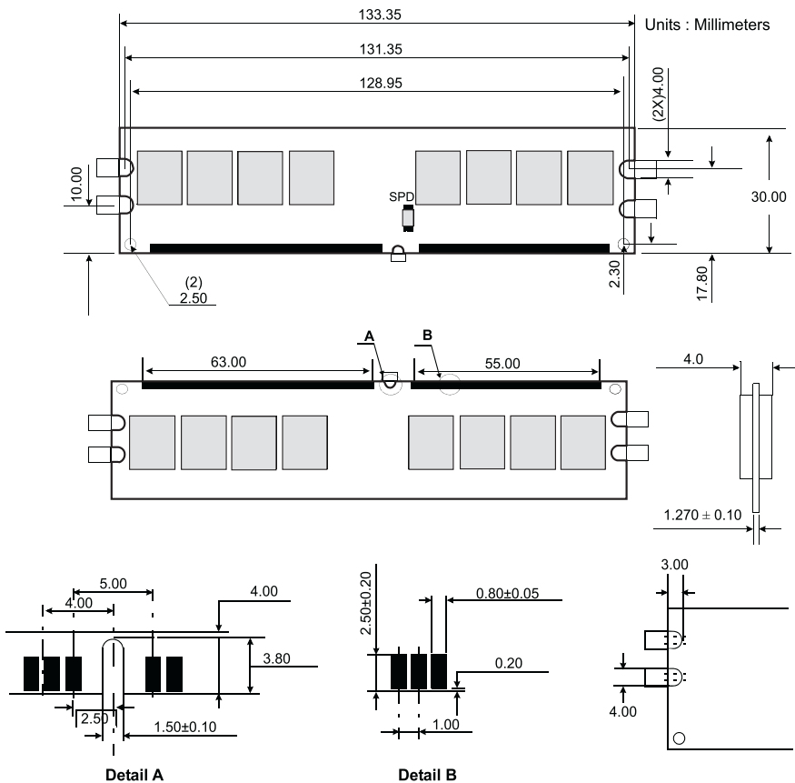
Figure 1: KVR400D2N3/2G 240-Pin DIMM
