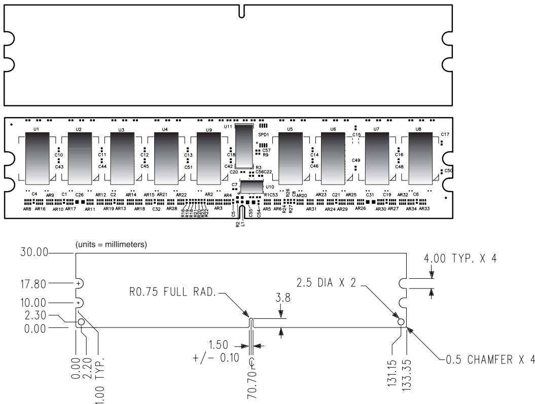
Figure 1: KVR400D2S8R3/1G 240-Pin DIMM
