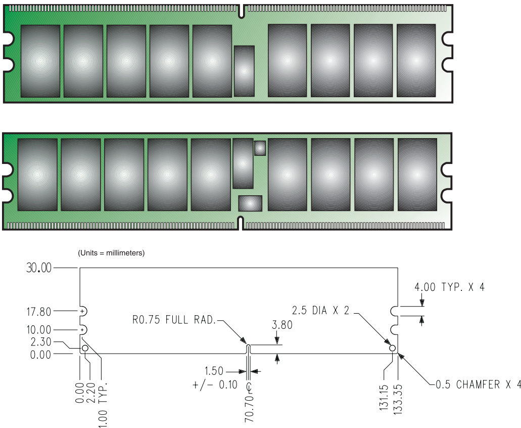
Figure 1: KVR667D2D8P5K2/4G 240-Pin DIMM
