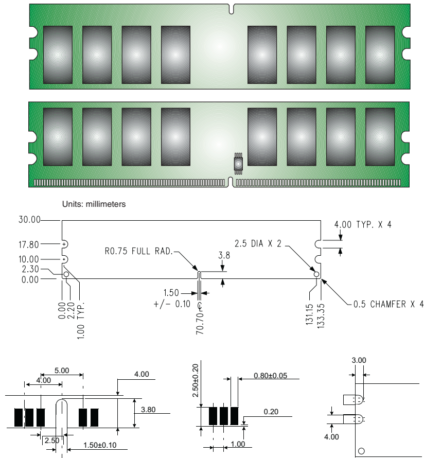
Figure 1: KVR667D2N5/4G 240-Pin DIMM
