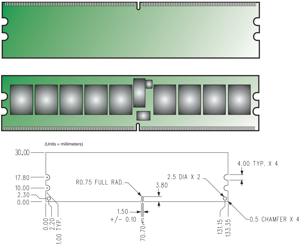
Figure 1: KVR667D2S8P5/1G 240-Pin DIMM
