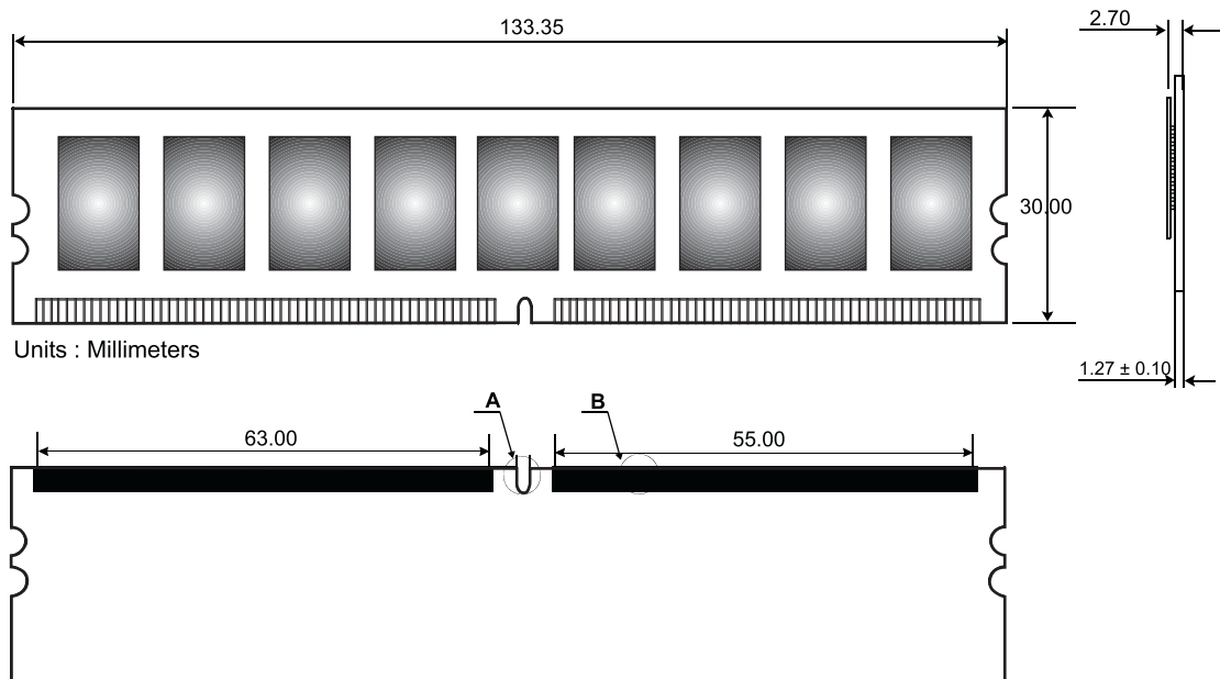
Figure 1: KVR800D2E6K2/2G 240-Pin DIMM
