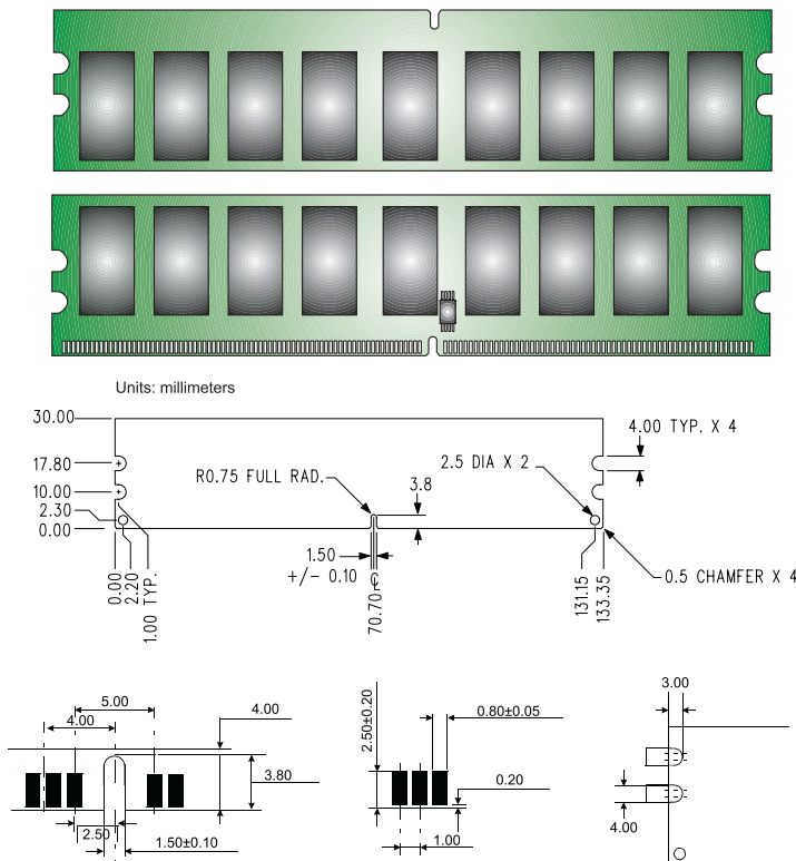
Figure 1: KVR800D2E6K2/4G 240-Pin DIMM
