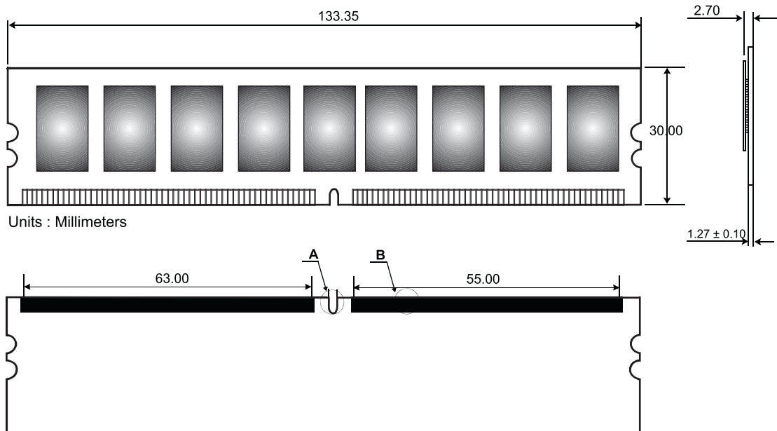
Figure 1: KVR800D2E6/1G 240-Pin DIMM
