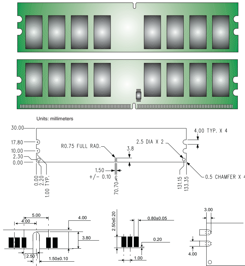
Figure 1: KVR800D2N6K2/8G 240-Pin DIMM Kit
