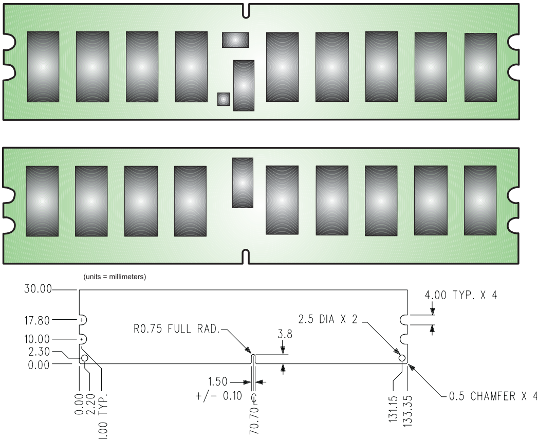
Figure 1: KVR800D2S4P6/2G 240-Pin DIMM
