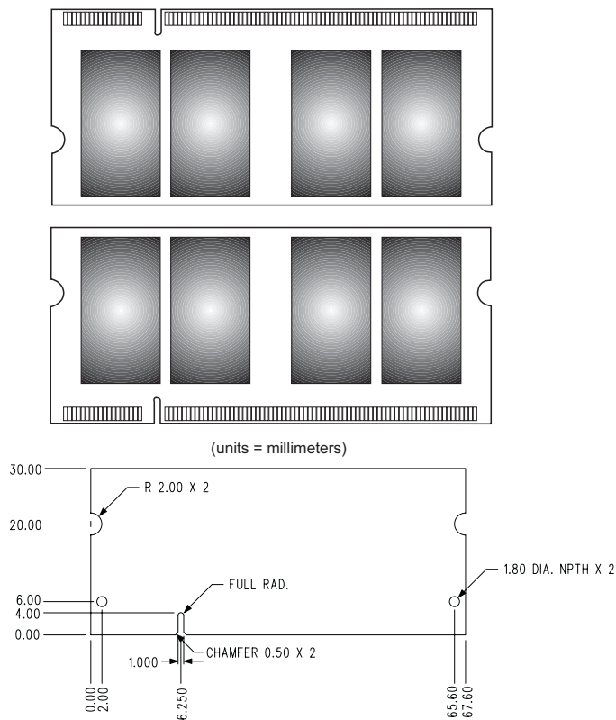
Figure 1: KVR800D2S6K2/2G 200-Pin SODIMM
