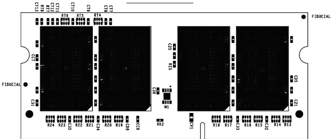
PRIMARY SIDE
